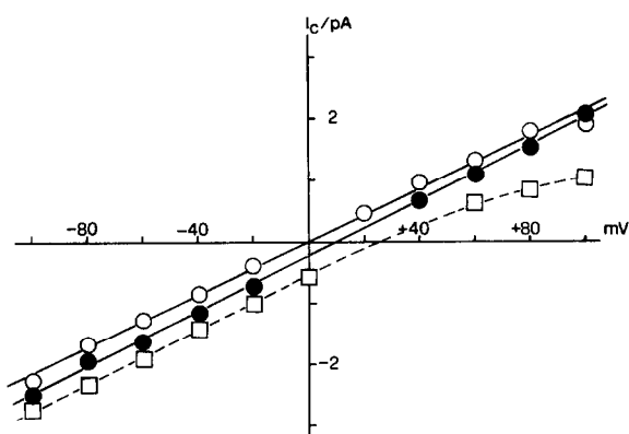
Fig.2. Current-voltage relationships for a cation channel in an inside-out patch. The bath and the pipette initially contained 130 mM NaCl symmetrical (A1) solution ( \circ ). The bath solution was subsequently replaced with 40 mM NaCl (A2) solution ( \square ) and 130 mM KCl (B1) solution ( \bullet ).
